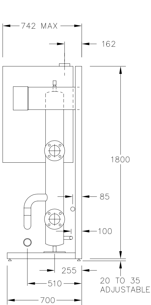
VIEW A
