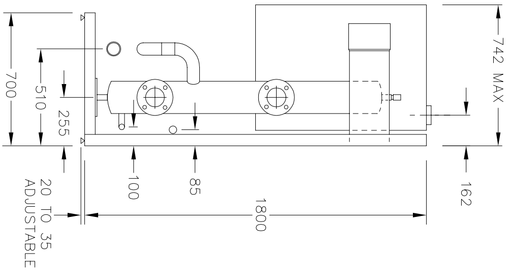
VIEW A BOILER PIPEWORK OMITTED FOR CLARITY
